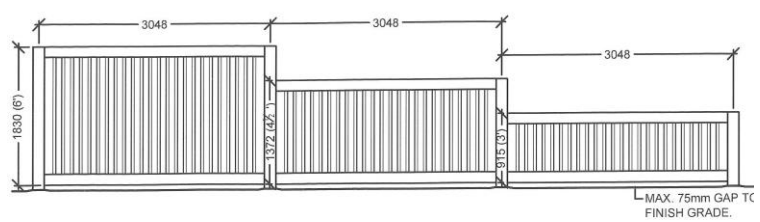
2 OVERLAP WOOD SCREEN FENCE STEP DOWN SCALE: 1:50
