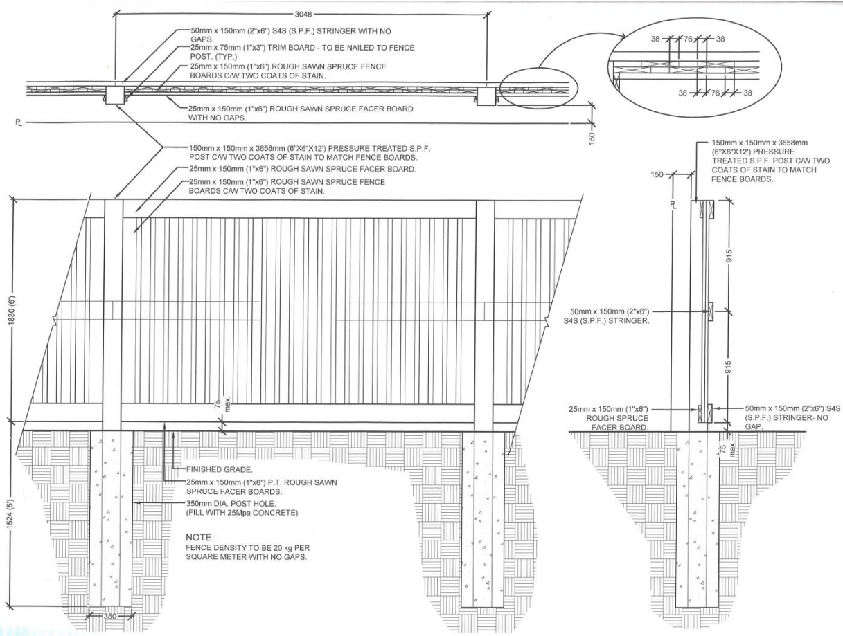
1 1800mm HT. OVERLAP WOOD SCREEN FENCE SCALE: 1:20
