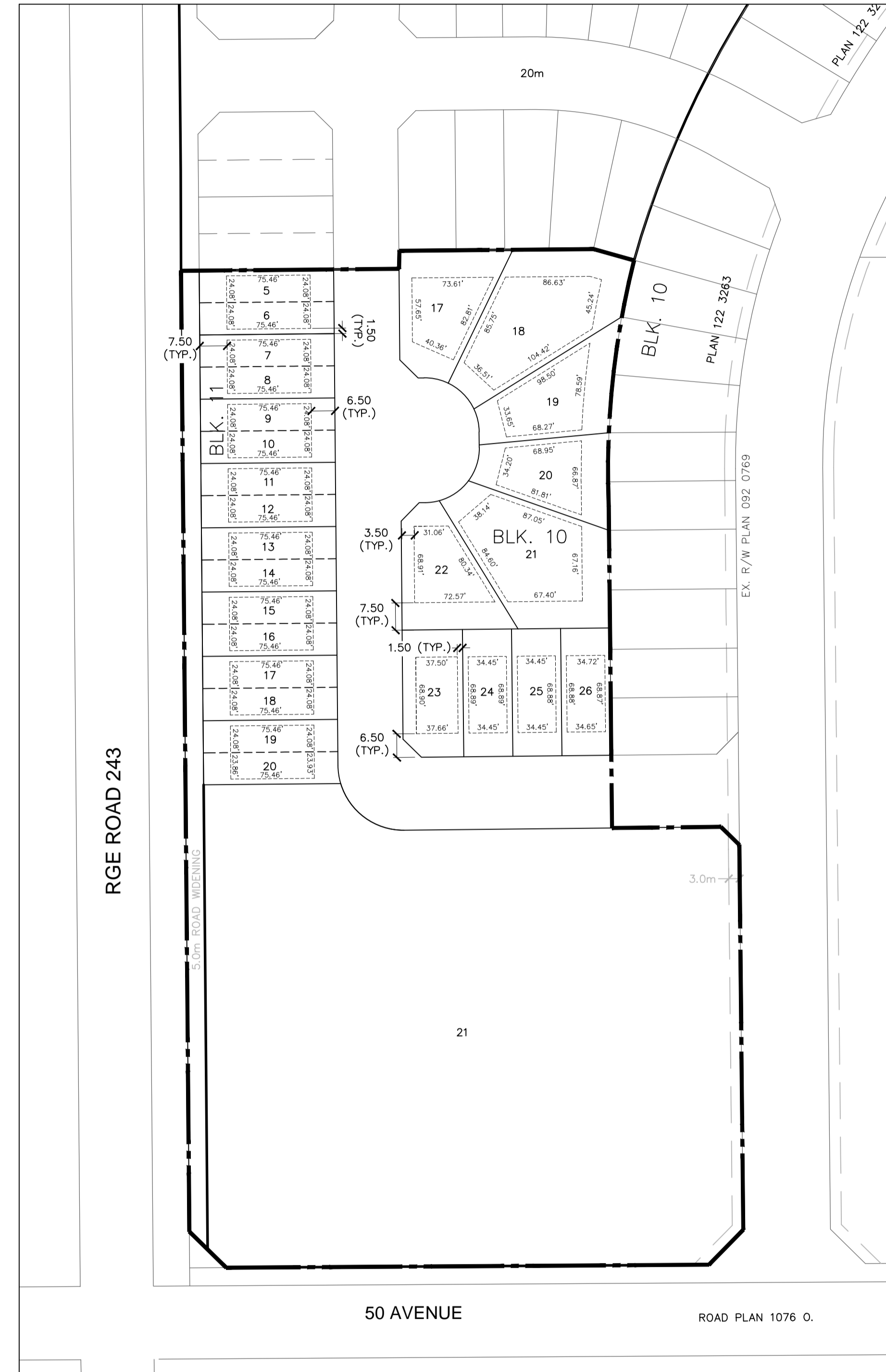
PHASE 6 (SOUTH) 1:1000
