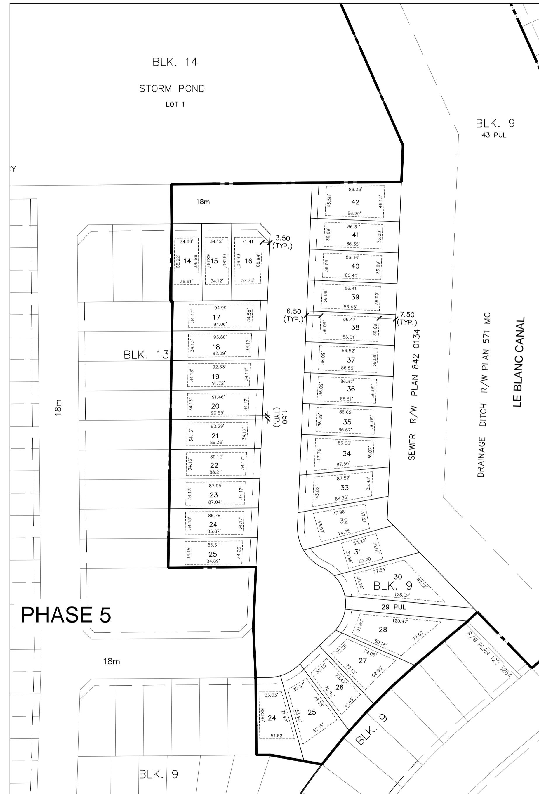
PHASE 6 (NORTH) 1:1000
